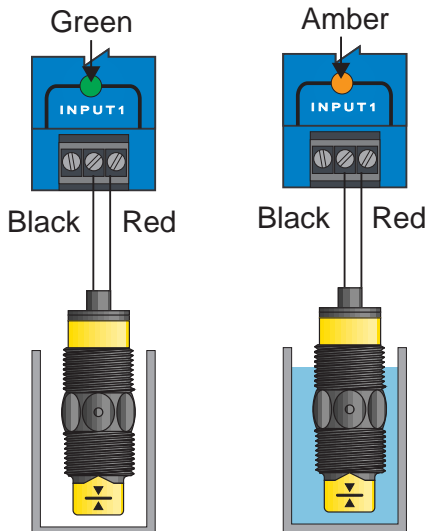
Wiring to a Powered Switch
