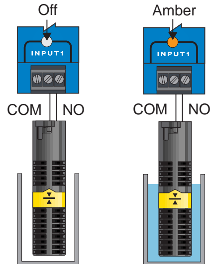
Wiring to a Mechanical Switch
