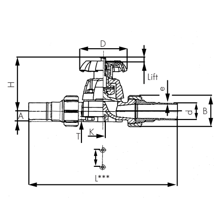
BCF fusion end connections
