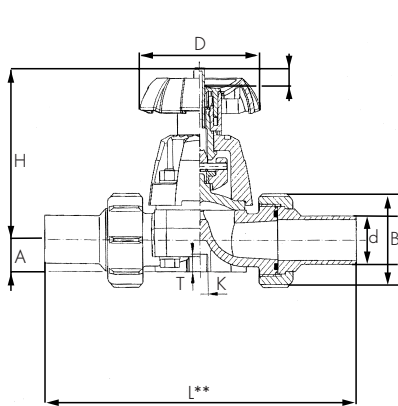
IR/butt fusion end connections
